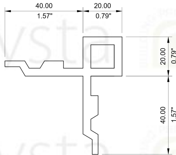
2 FRONT ELEVATION DC-1 SCALE 1:1
