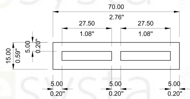
2 FRONT ELEVATION C-6 SCALE 1:1
