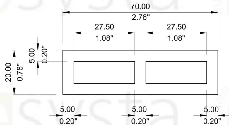
2 FRONT ELEVATION C-5 SCALE 1:1
