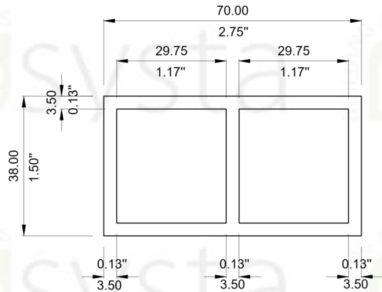
2 FRONT ELEVATION C-1 SCALE 1:1
