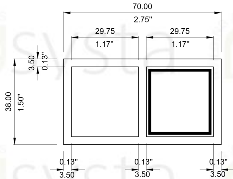
2 FRONT ELEVATION C-2 SCALE 1:1
